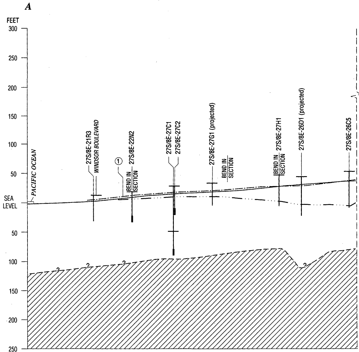
A. Santa Rosa Basin
