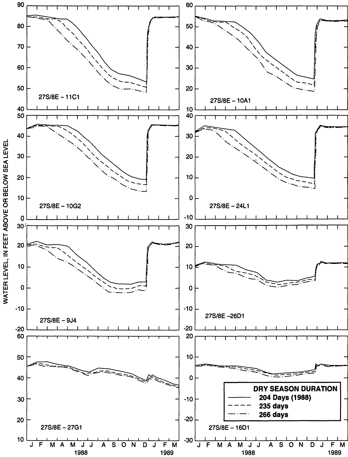
Figure 26. Effects of dry-season duration on simulated ground-water levels for the Santa Rosa and the San Simeon ground-water basins, San Luis Obispo County, California, 1988-89—Continued.
