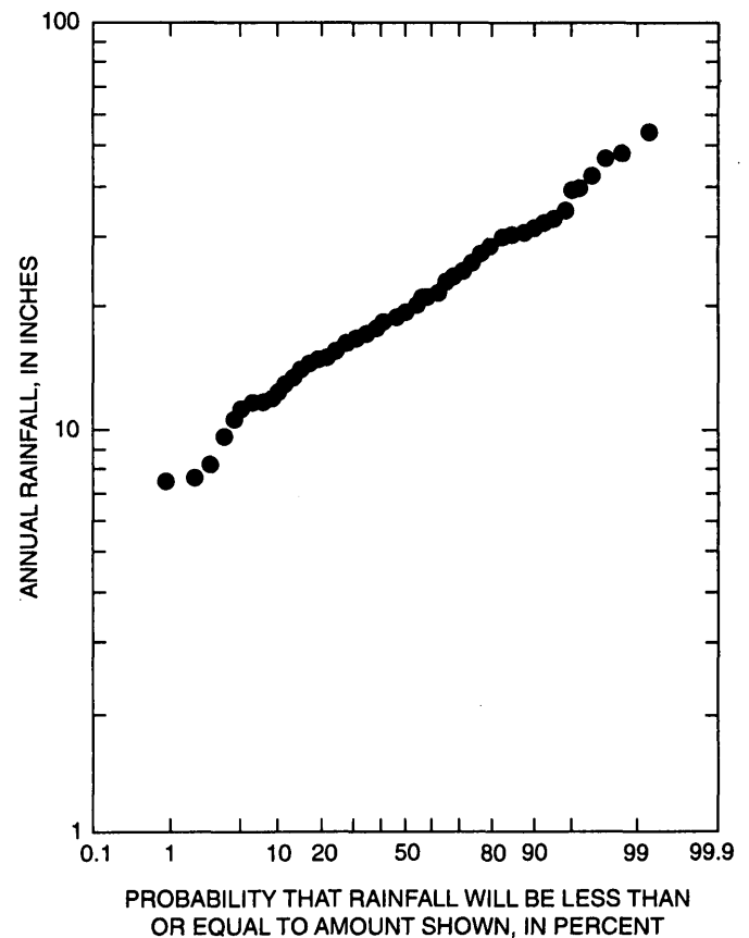
Figure 28. Probability distribution of annual rainfall at the San Luis Obispo-Poly station, San Luis Obispo County, California, 1870–1989.
