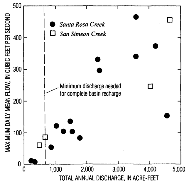
Figure 29. Relation of maximum daily mean flow and annual discharge in Santa Rosa and San Simeon Creeks, San Luis Obispo County, California.
